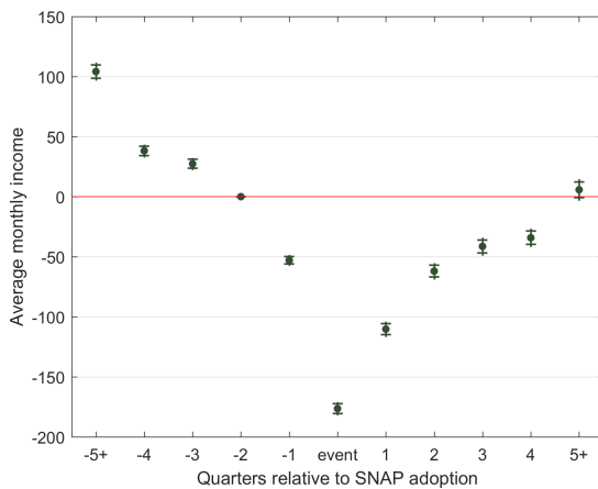
Figure 7: Estimated changes in household income at quarters around SNAP adoption. Each figure plots estimates of coefficients \delta from (15), with the time period two quarters prior to SNAP adoption (“-2”) as the omitted category. Inner confidence sets as indicated by the dashes correspond to 95% pointwise confidence intervals, while outer confidence sets are the uniform 95% sup-t bands (with critical values obtained via simulation). Standard errors are clustered at the household level.
