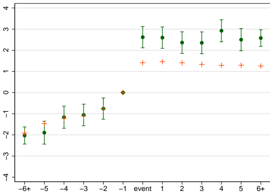
(c) Overlaying outcome of interest (with confidence intervals) y_{it} and unaffected covariate x_{it} (+, rescaled) around event time.
