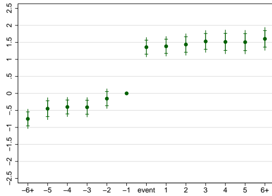
(e) Pre-testing for trend
