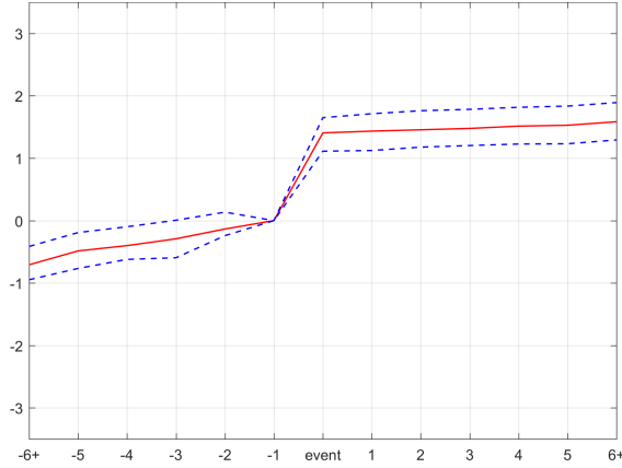
(e) Pre-testing for pre-trend. Ignoring \eta_{it} if no pre-trend accepted. Estimates based on the 584 realisations with no detected pre-trend.
